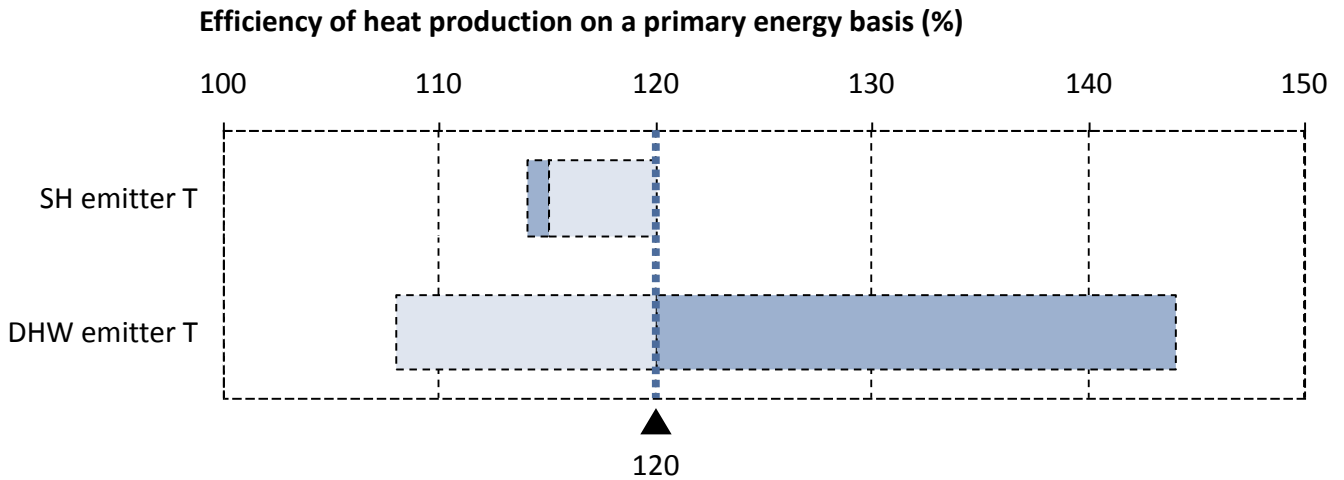
Figure 30: Impact of emitter temperatures on efficiency of heat production on a primary energy basis for Scenario 3. The thick blue line indicates value using the Central sensitivity assumptions. The darker bars represent the Low sensitivity assumptions, and the lighter bars the High sensitivity assumptions, as shown in Table 14.
