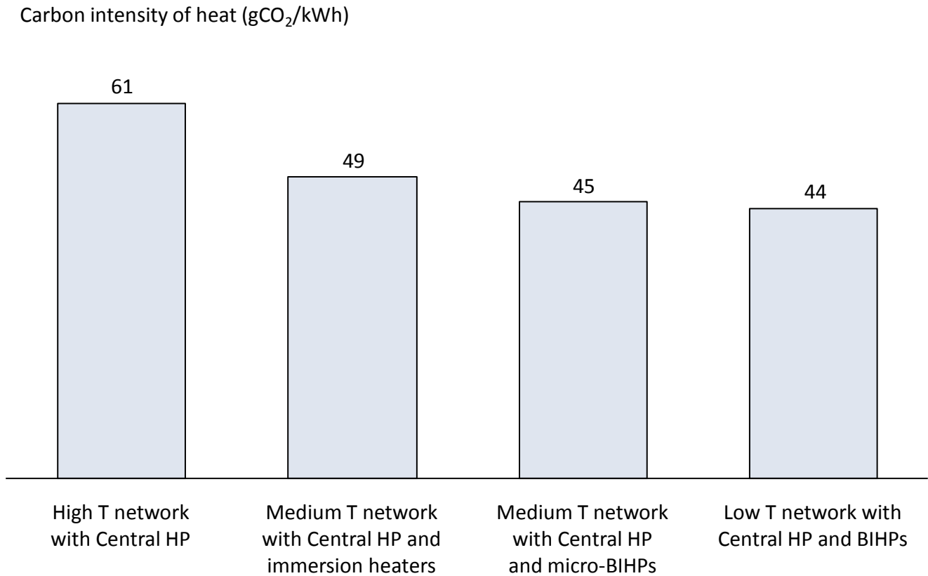
Figure 42: Comparison of CO 2 emissions for the different HP in DH schemes studied in Demand Case A.
