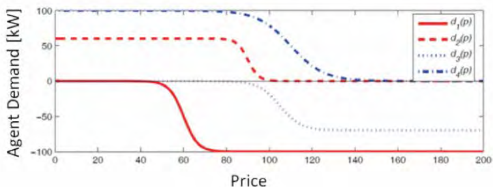
Bid curves offered by the agents to the auctioneer agent
