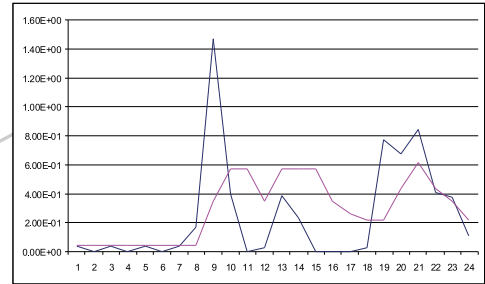
load profiles
